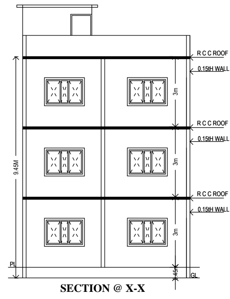
SECTION @ X-X
